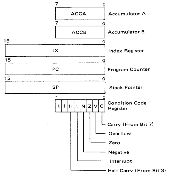
FIGURE 14 — PROGRAMMING MODEL OF THE MICROPROCESSING UNIT
