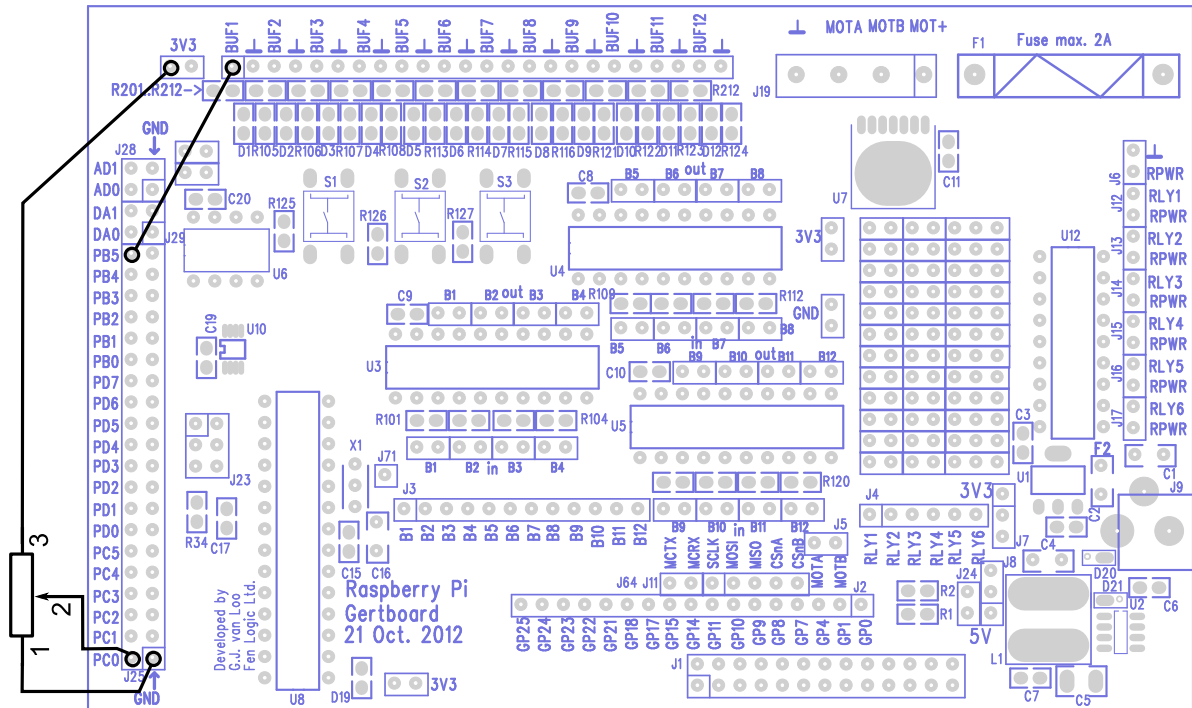
Figure 32: Wiring diagram for the AnalogInput sketch.
