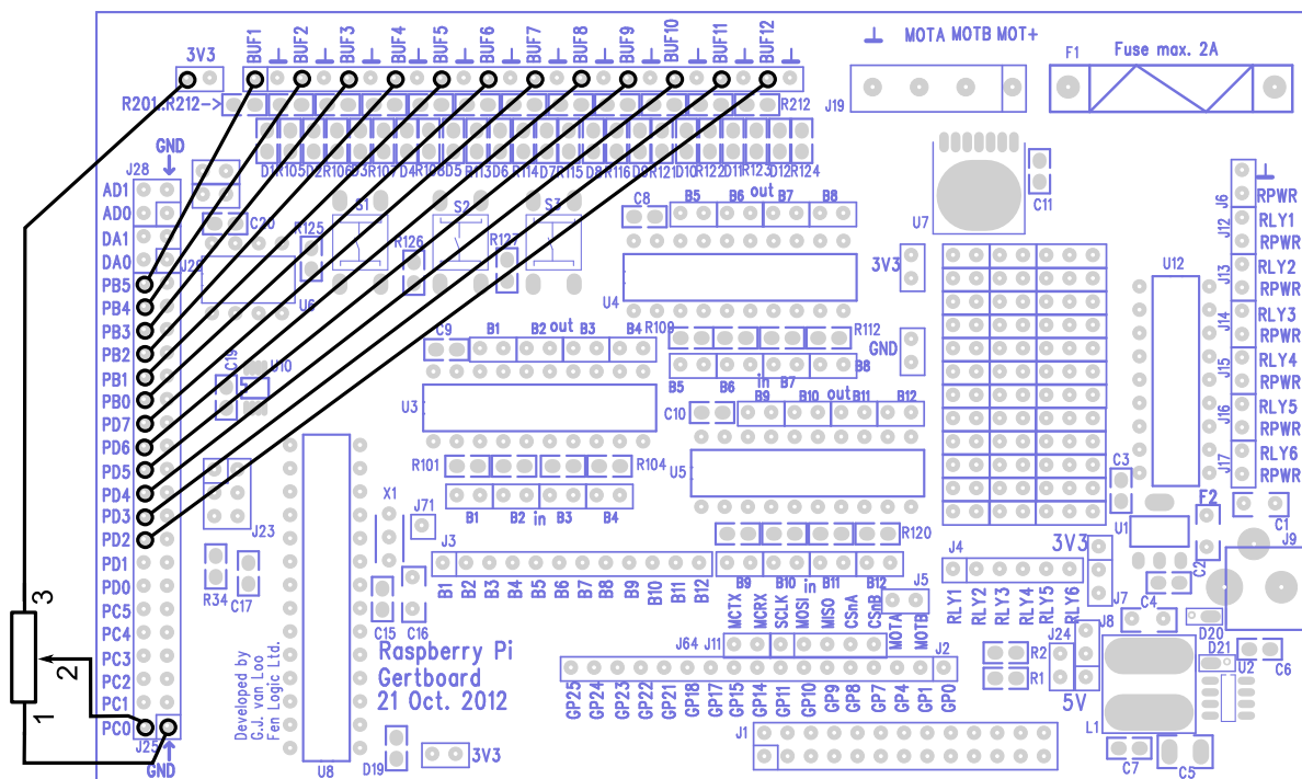
Figure 34: Wiring diagram for the LEDmeter sketch
