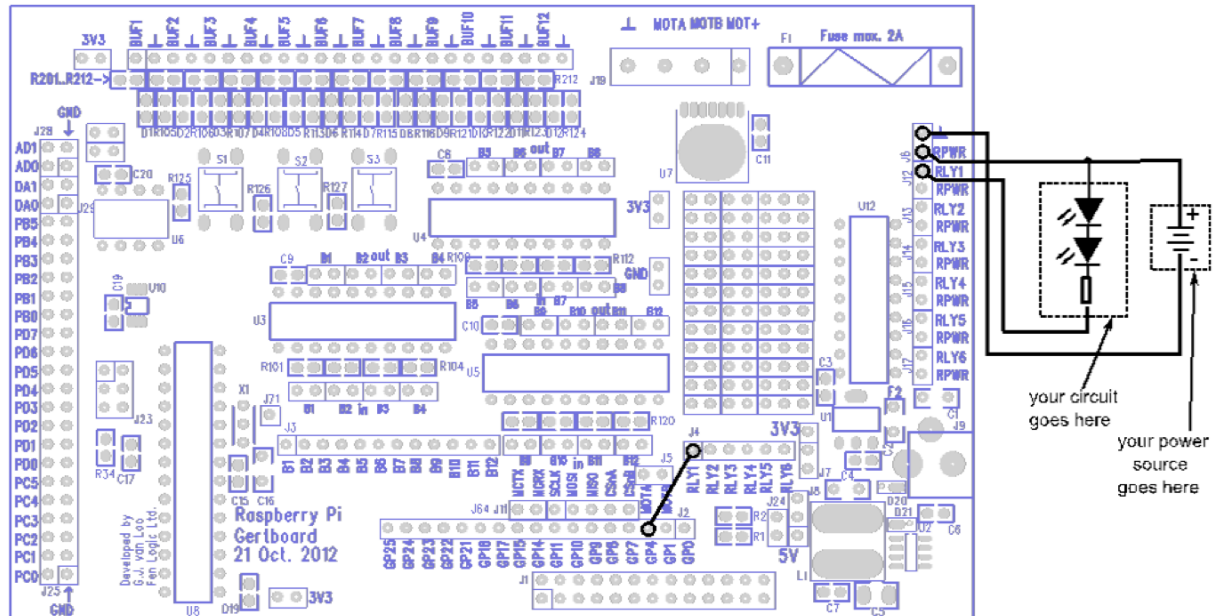
Figure 16: Wiring diagram to test the open collector drivers. On the right is a small test circuit made up of two LEDs in series with a 90 Ω resistor, and a 9V battery acting as power supply.
