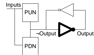
Fig. 1. Basic structure of a component required for asynchronous circuits.
