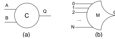
Figure 2 – (a) Symbol of a 2-input C-element and (b) symbol of an M-of-N gate.
