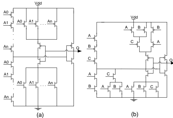
Figure 3 – Examples of NCL gates: (a) an N-of-N NCL gate, or a C-element; (b) 2-of-3 NCL gate [5].
